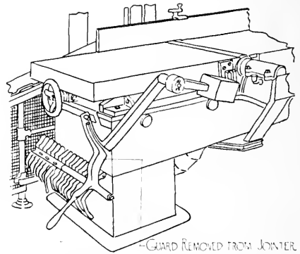
—GUARD REMOVED FROM JOINTER FIG. 151. JOINTER GUARD REMOVED.
